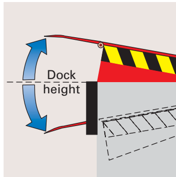
Operating range above and below dock height
